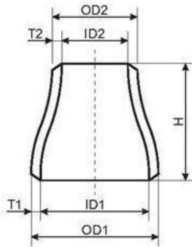
Large-Caliber Seamless WP 321 Concentric Carbon Steel Reducer
