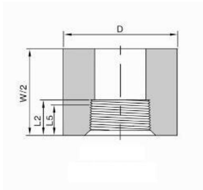
High press Forged Pipe Fitting Half Coupling
