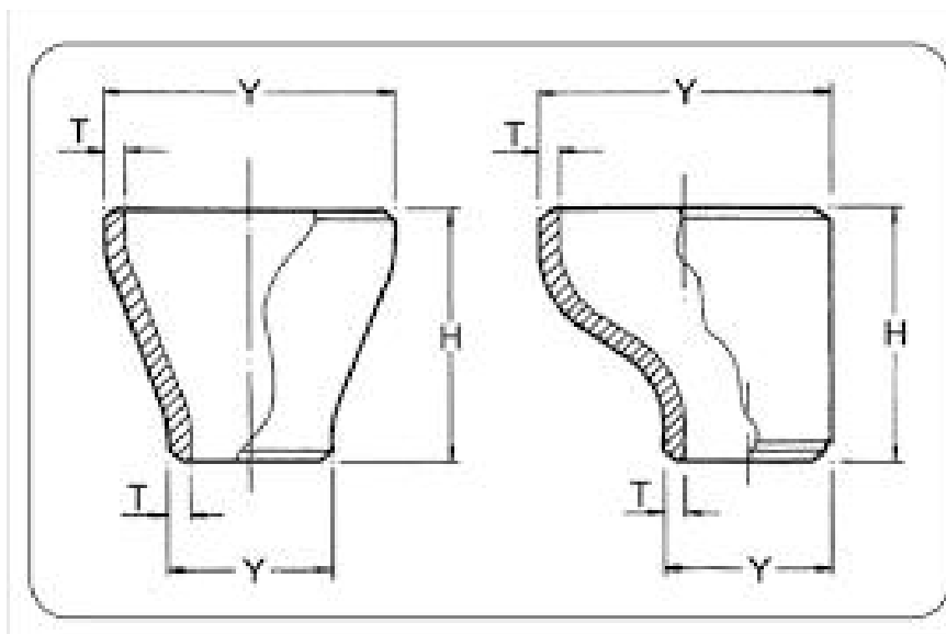
large-caliber pipe fitting reducer
